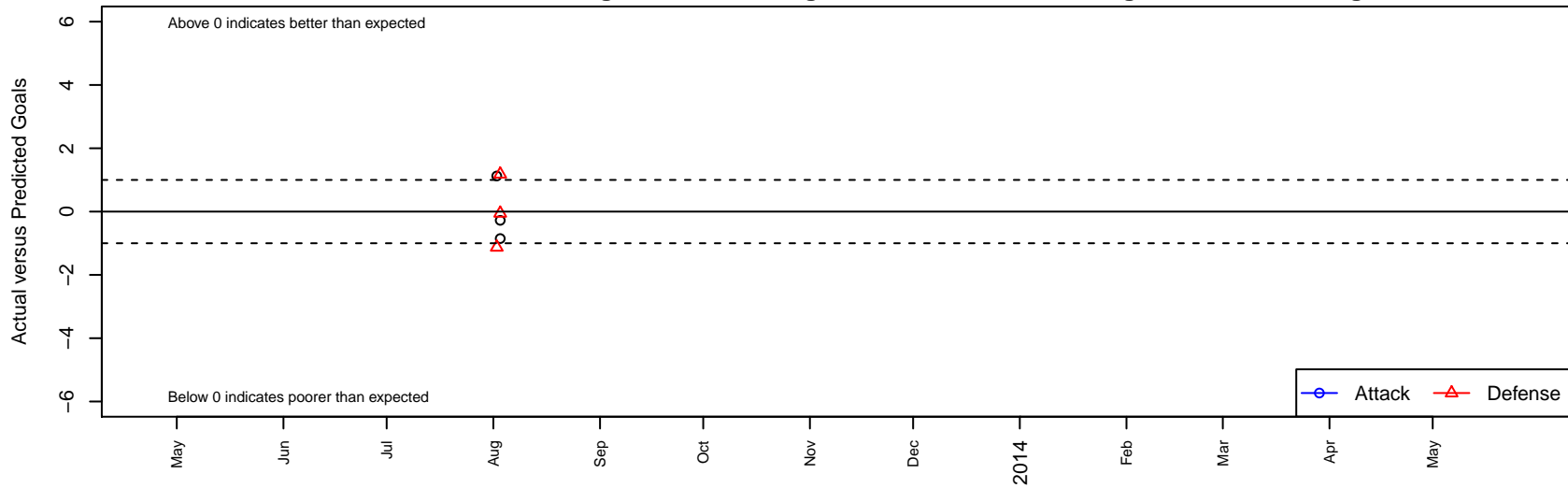
Elko Indar G99 Dots are actual minus expected GF (blue circles) and GA (red triangles). Blue line is smoothed change in attack strength. Red is smoothed change in defense strength.
